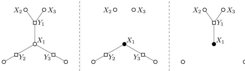
FIGURE 2: (a) A directed graphical model G . The cavity models (b) G_{X_1 \rightarrow Y_1} and (c) G_{Y_1 \rightarrow X_1} .
